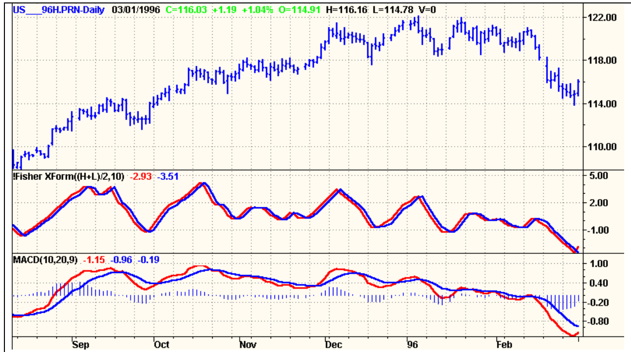
Figure 5. The Fisher Transform of Normalized Prices Has Very Sharp Turning Points When Compared to Conventional Indicators such as the MACD
